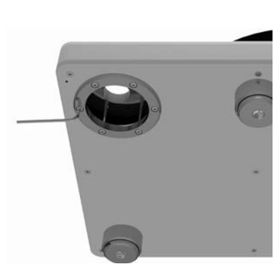
Pic. 3b: Mounting of the tonarm base on the bottom side
